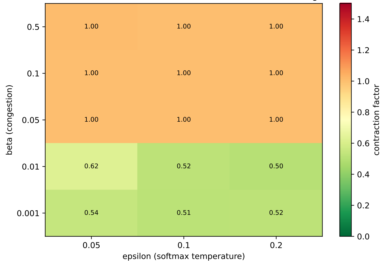
EXP-12 contraction factor c ( \lambda=0.5 ); c < 1 = converges
