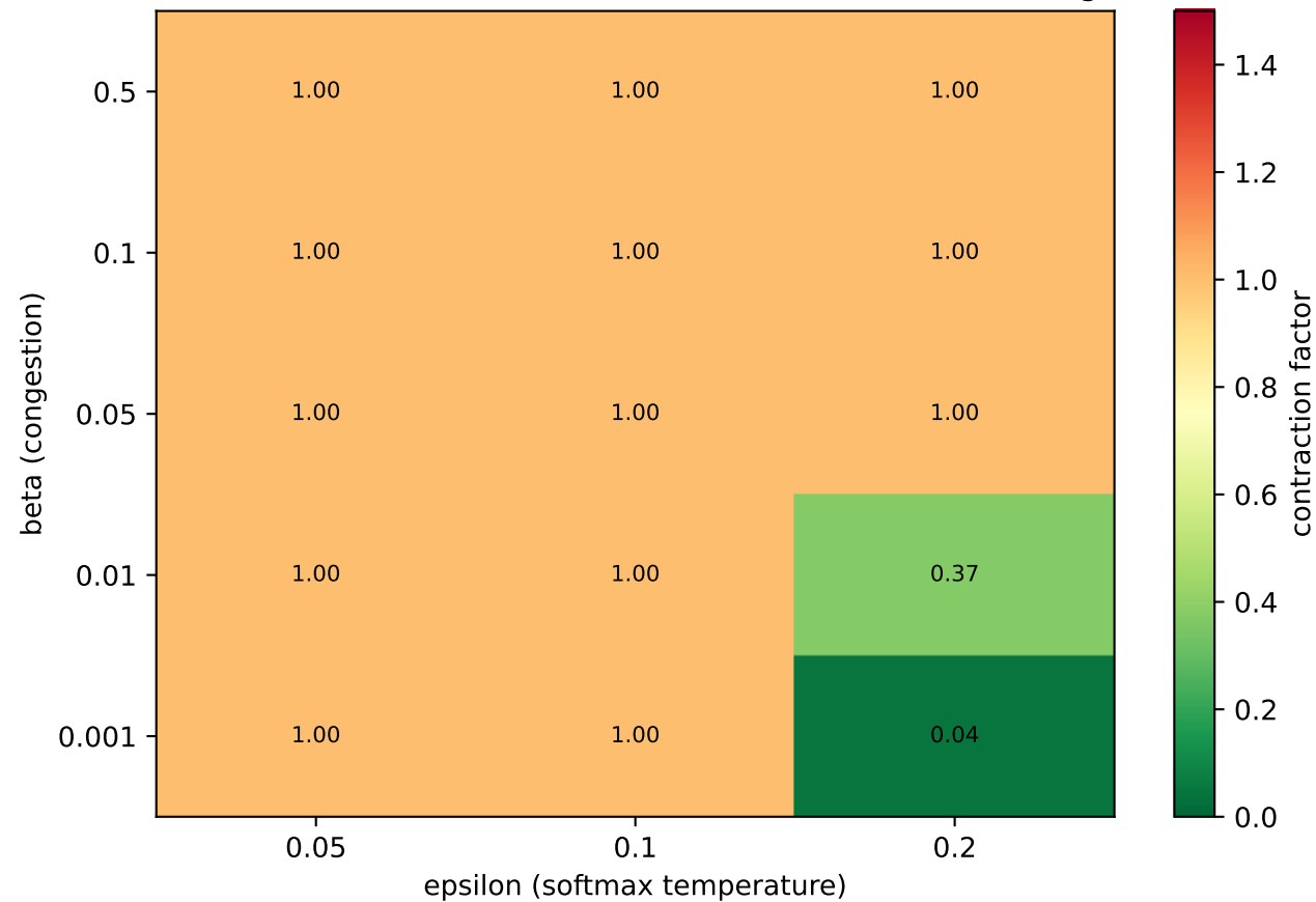
EXP-12 contraction factor c ( \lambda=1.0 ); c < 1 = converges
