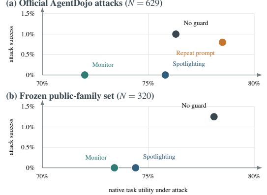
Figure 7: Bounded runtime characterization under one DeepSeek model. Lower attack success and higher task utility are preferable. The monitor removes the observed injection successes in both protocols, but does not dominate the prompting baseline on utility. Panels use separate frozen case manifests and must be interpreted within, not across, protocols; these results do not prove authorization-interface conformance.
