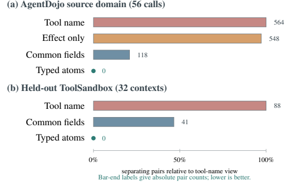
Figure 3: Representation collision falls as the authorization view preserves execution-relevant effects. Bars normalize policy-separating pair counts to the tool-name view within each domain; labels report absolute counts. Typed atoms reach the source-effect partition in both the development and held-out domains.
