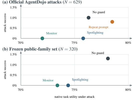
Figure 4: Security-utility tradeoff under one DeepSeek model. Lower attack success and higher task utility are preferable. The monitor removes the observed injection successes in both protocols, but does not dominate the prompting baseline on utility. Panels use separate frozen case manifests and must be interpreted within, not across, protocols.
