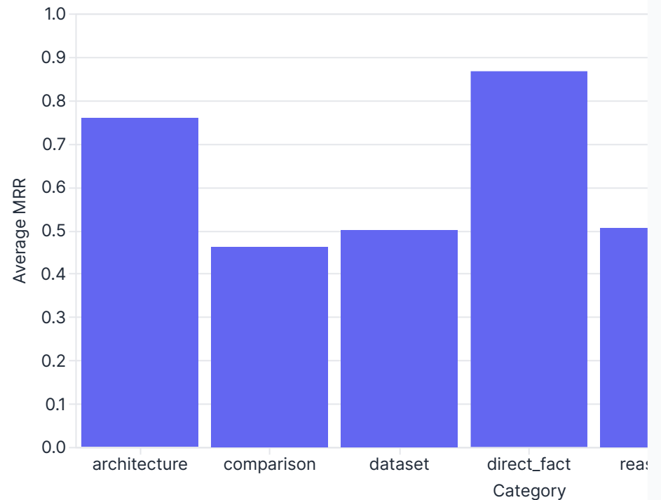
Average MRR by Category
