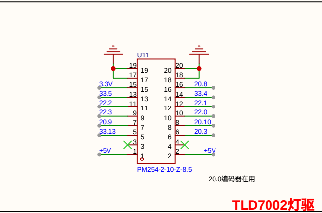
TLD7002灯驱
