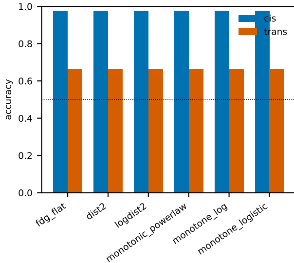
Same/cross
