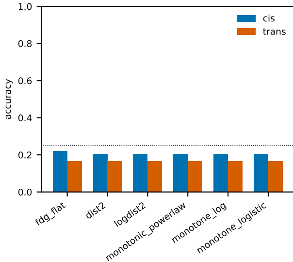
Exact four-state
