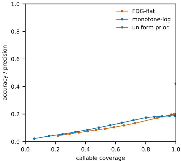
Exact state
