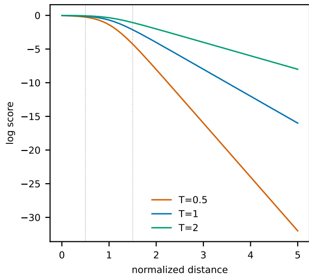
monotone_logistic
