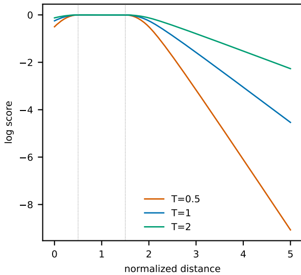
logdist2
