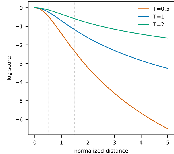
monotone_logistic
