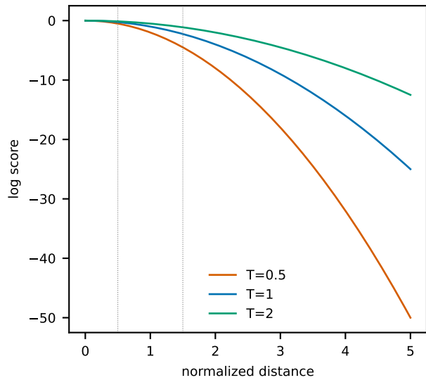
monotonic_powerlaw
