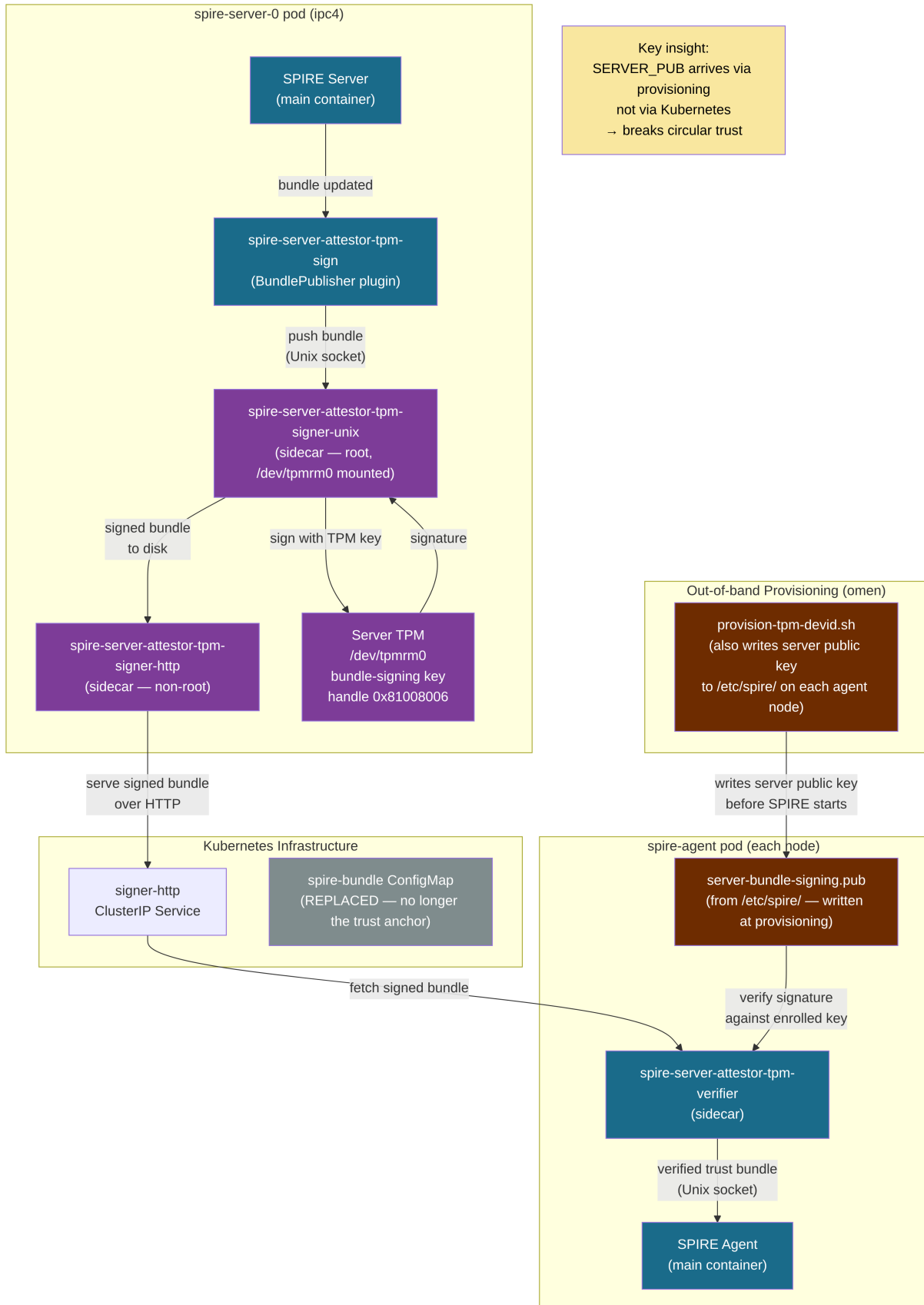
Figure 4: TPM server bundle signing and verification flow
