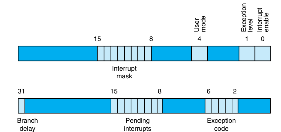
FIGURE 8.13 The Cause and Status registers. This version of the Cause register corresponds to the MIPS-32 architecture. The earlier MIPS I architecture had three nested sets of kernel/user and interrupt enable bits to support nested interrupts. Section A.7 in Appendix A has more details about these registers.
