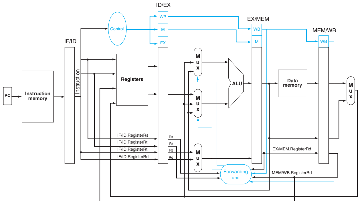
FIGURE 6.32 The datapath modified to resolve hazards via forwarding. Compared with the datapath in Figure 6.27 on page 404, the additions are the multiplexors to the inputs to the ALU. This figure is a more stylized drawing, however, leaving out details from the full datapath such as the branch hardware and the sign extension hardware.
