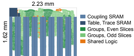
(a) Cell Placement
