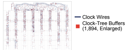
(c) Clock Tree
