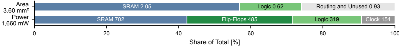
(d) Area and Power of One Engine at 1.25 GHz
