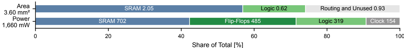
(d) Area and Power of One Engine at 1.25 GHz
