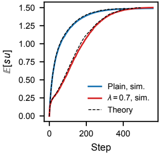
(a) Negative Energy per Spin
