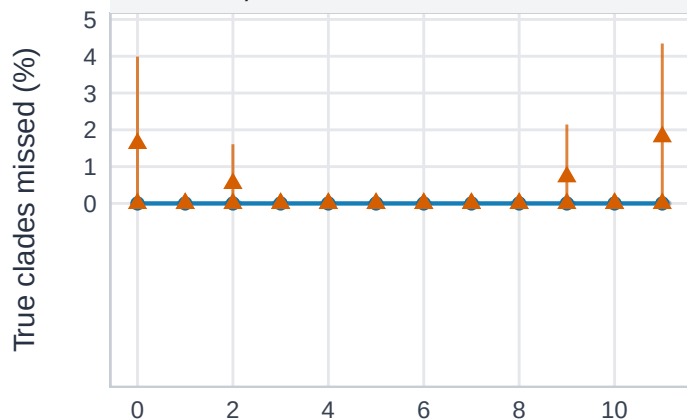
C Llama-3.2 decoder 16 blocks; n = 46
