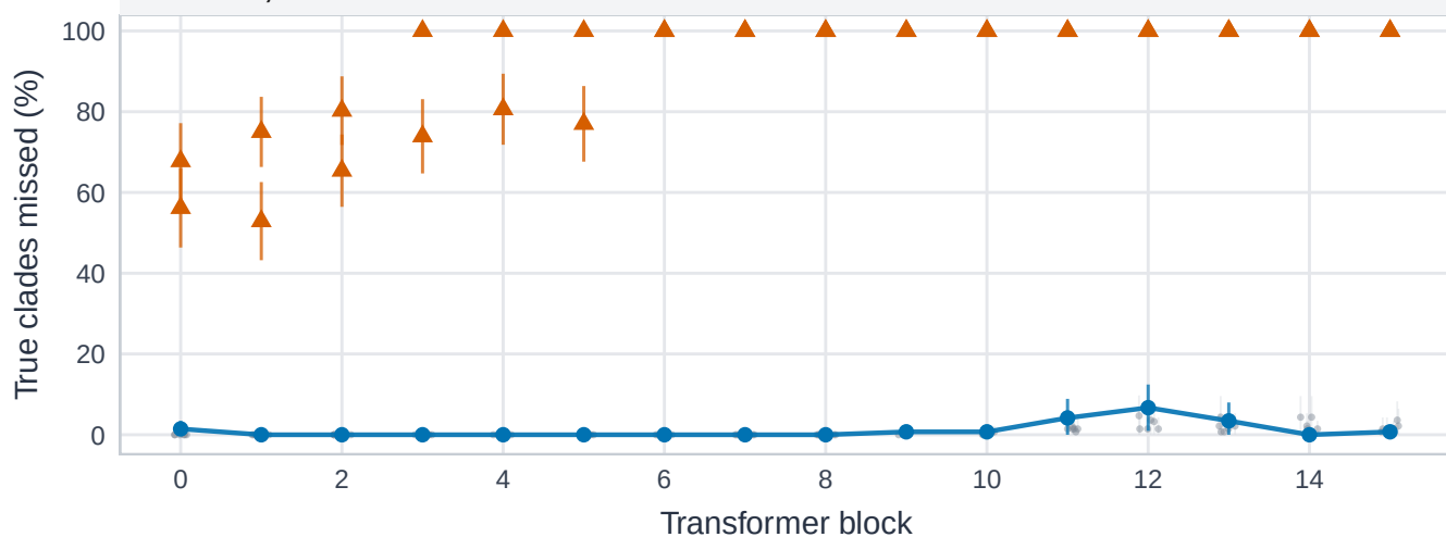
C Llama-3.2 decoder 16 blocks; n = 46
