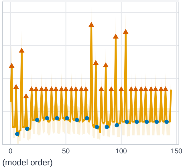
Llama-3.2-1B | decoder-only, d = 2048 n = 47; key matrices 13%, other layers 20% missed
