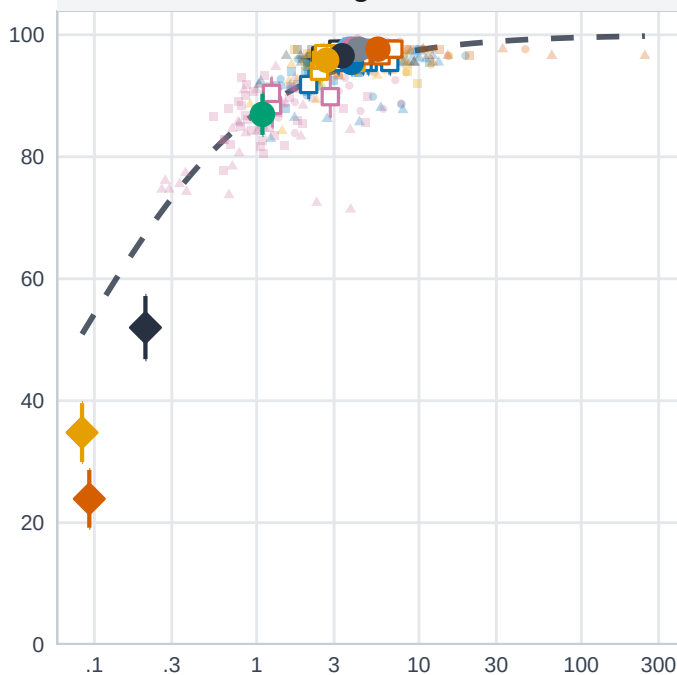
A Fitted Atteson diagnostic
