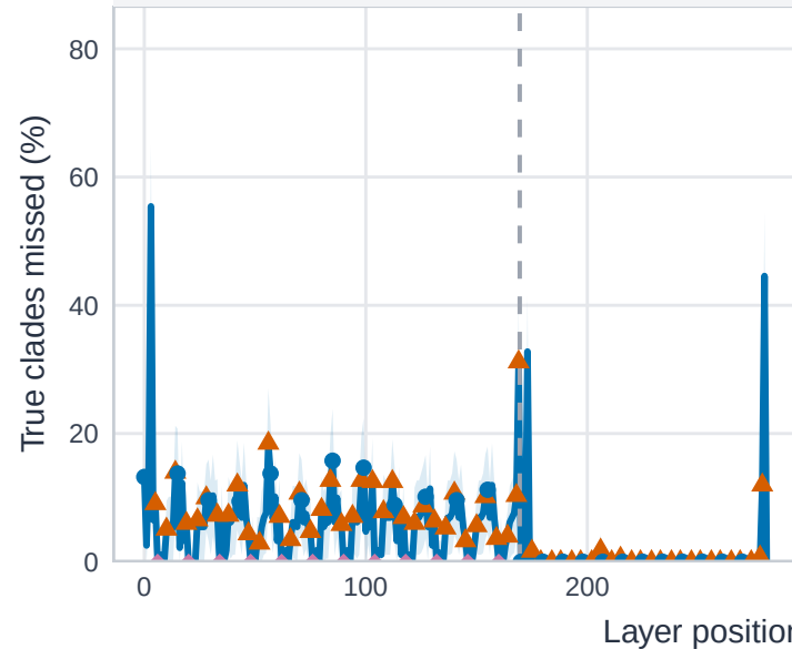
Flan-T5-base | encoder-decoder, d = 768 n = 46; decoder min 0% missed; 29/170 at ceiling
