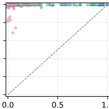
ARC-C
