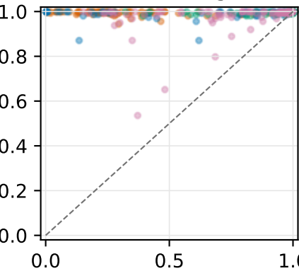
HellaSwag
