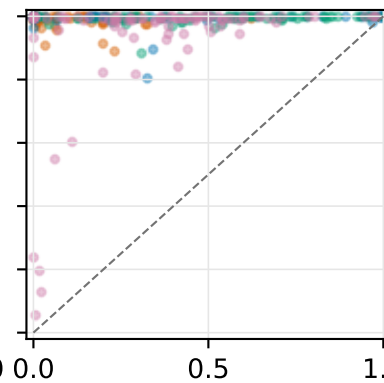
TruthfulQA
