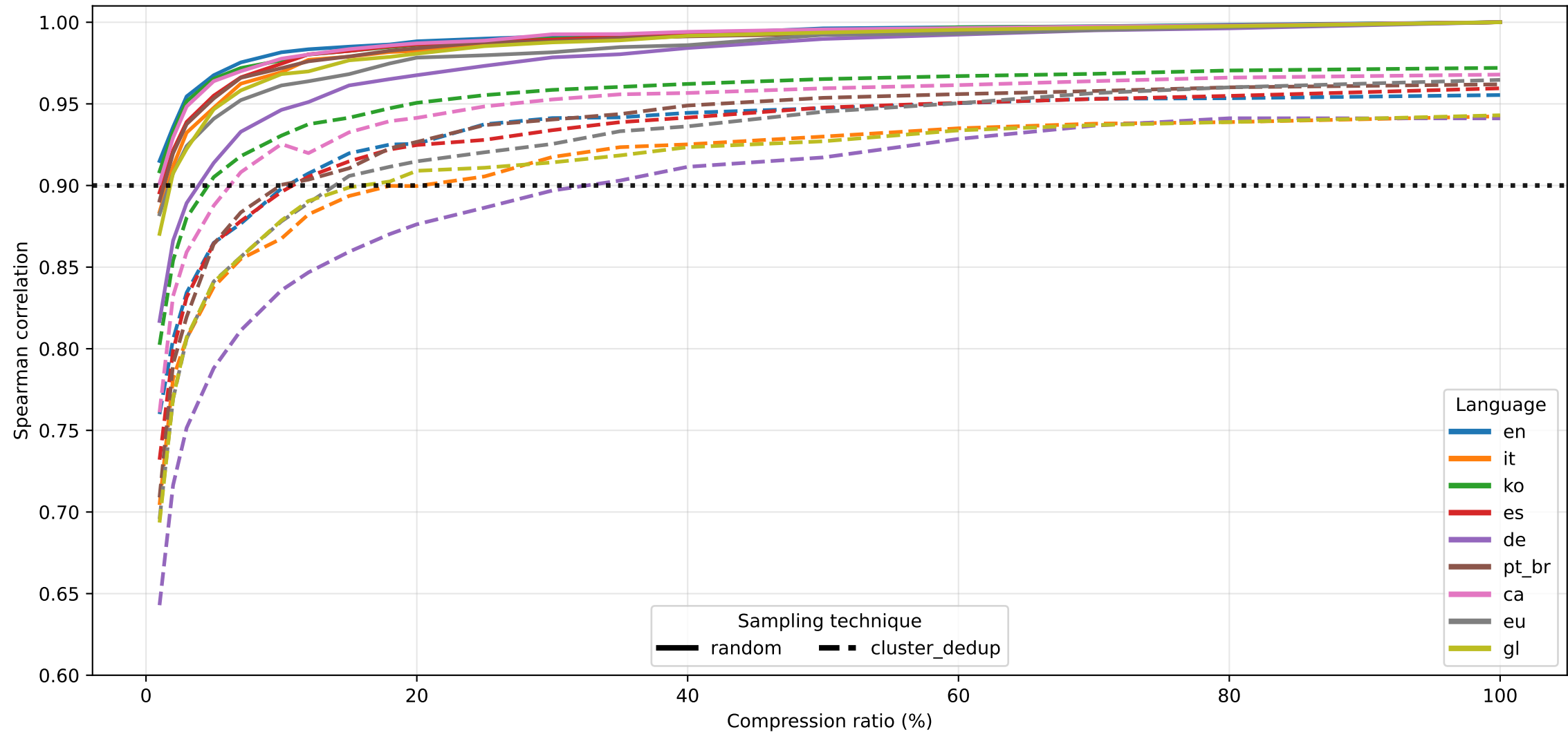
Sampling - Spearman correlation across languages
