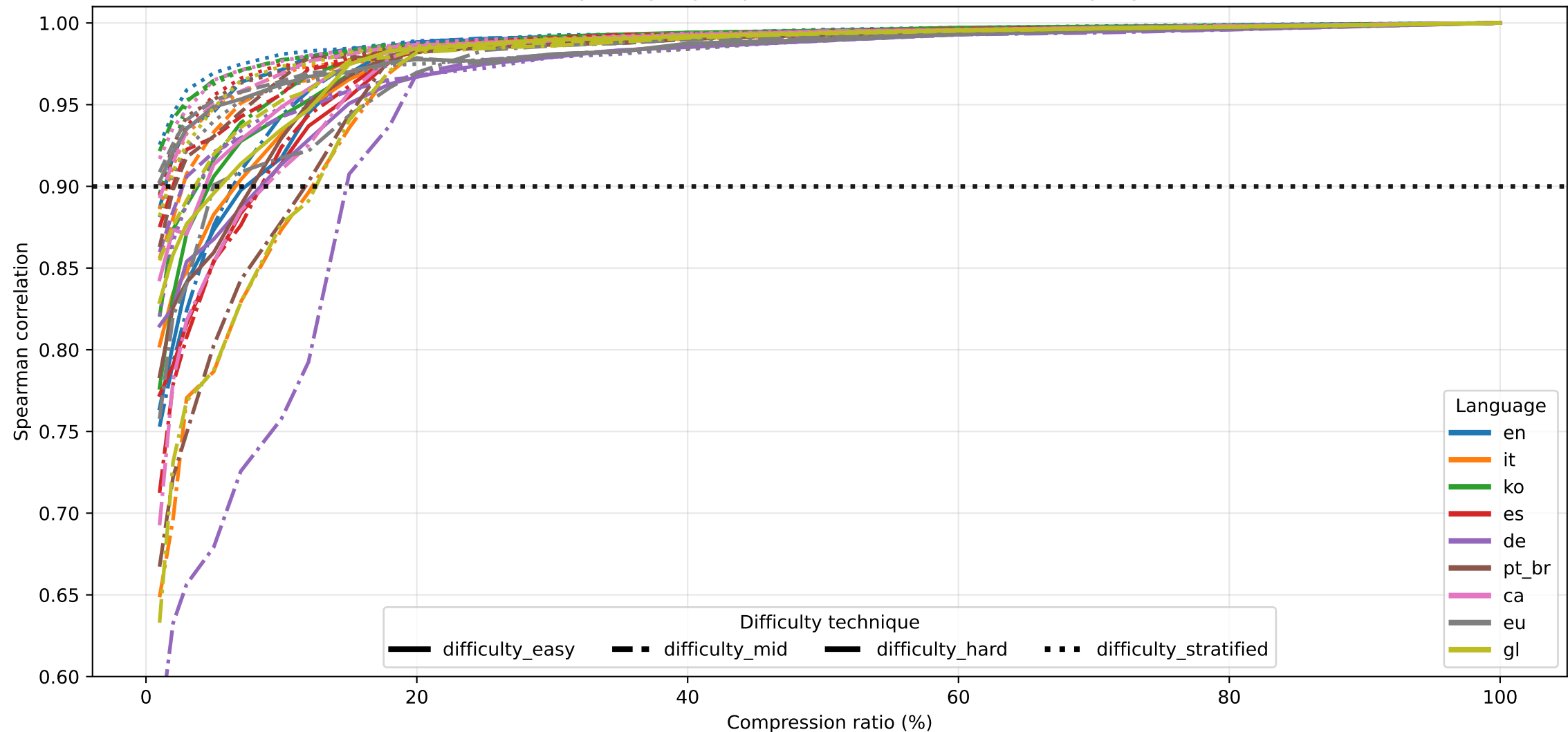
Difficulty Sampling - Spearman correlation across languages
