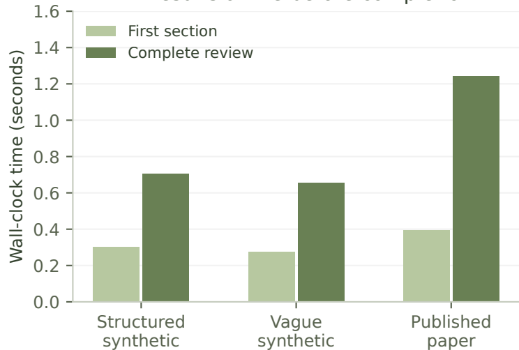
B. Results arrive before completion
