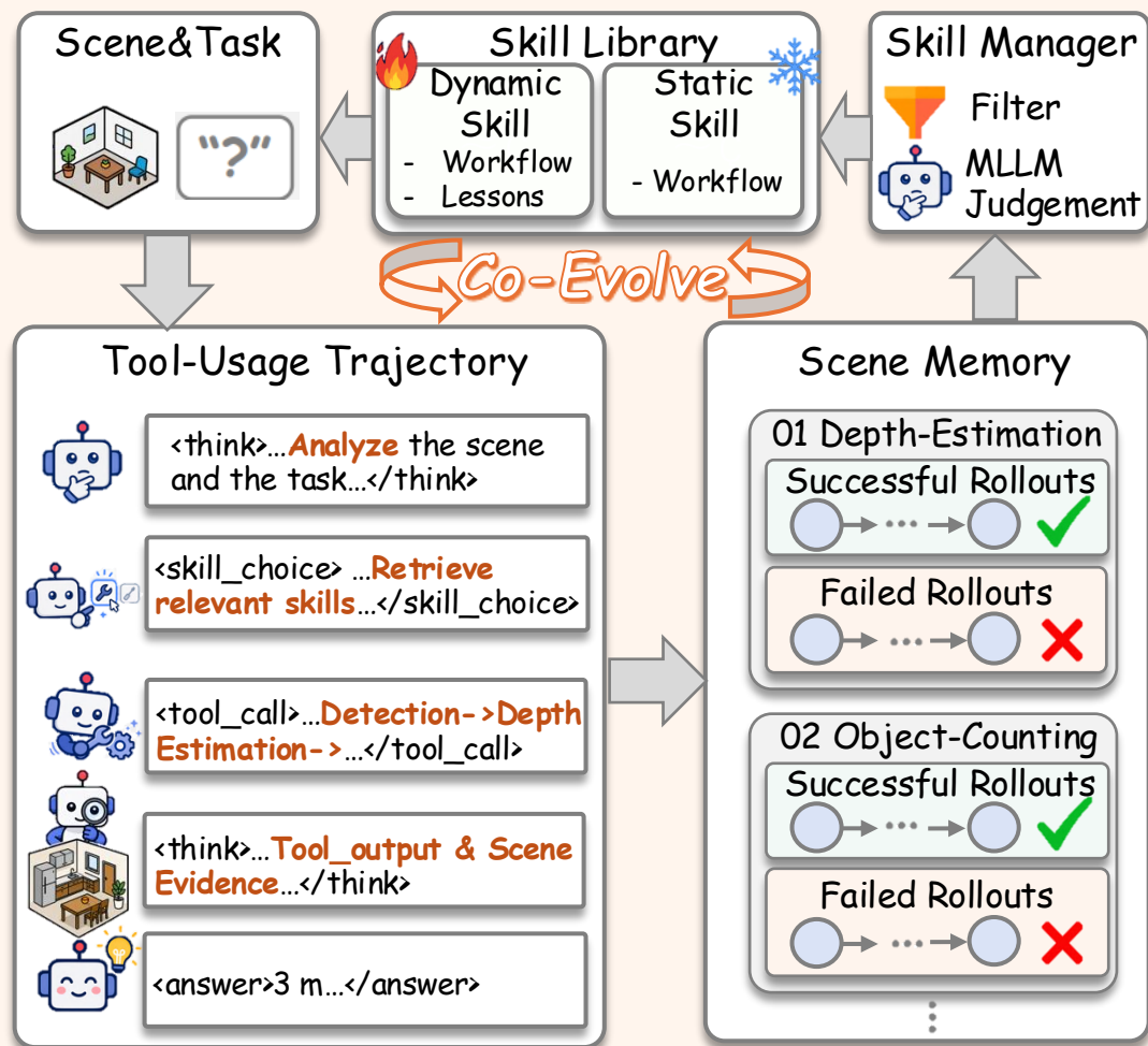
(a) Scene-Aware Skill Extraction
