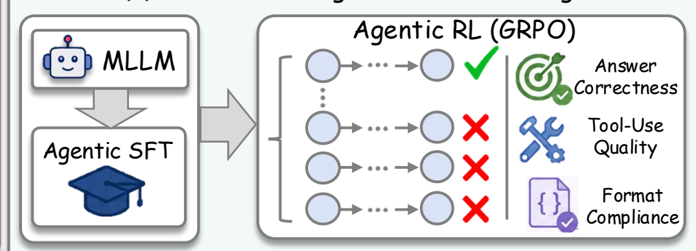
(c) Skill-Guided Agentic Post-Training
