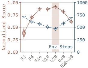
(a) Skill Durations
