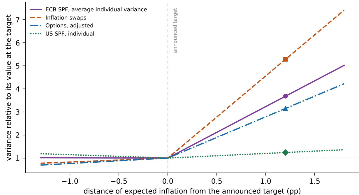
One law, four sources: flat below, rising above
