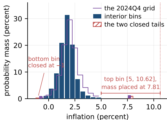
(b) average reported histogram, one year ahead
