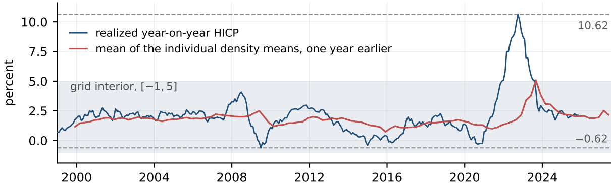
(a) realized one-year euro-area inflation and the average density mean
