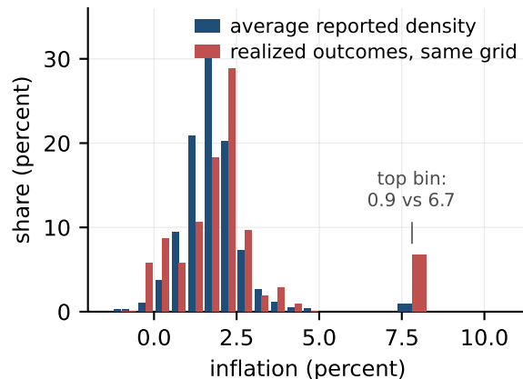
(c) the two histograms compared
