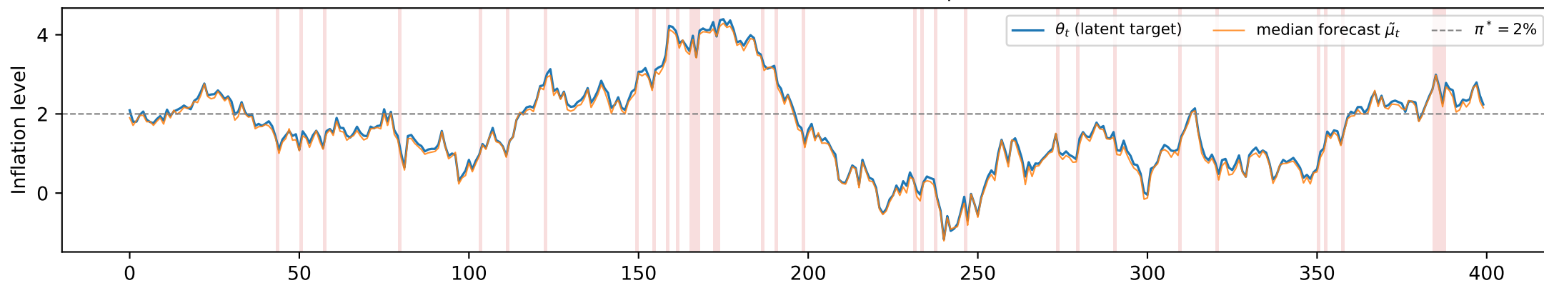
Panel A: First moment (levels) — artifact episodes shaded
