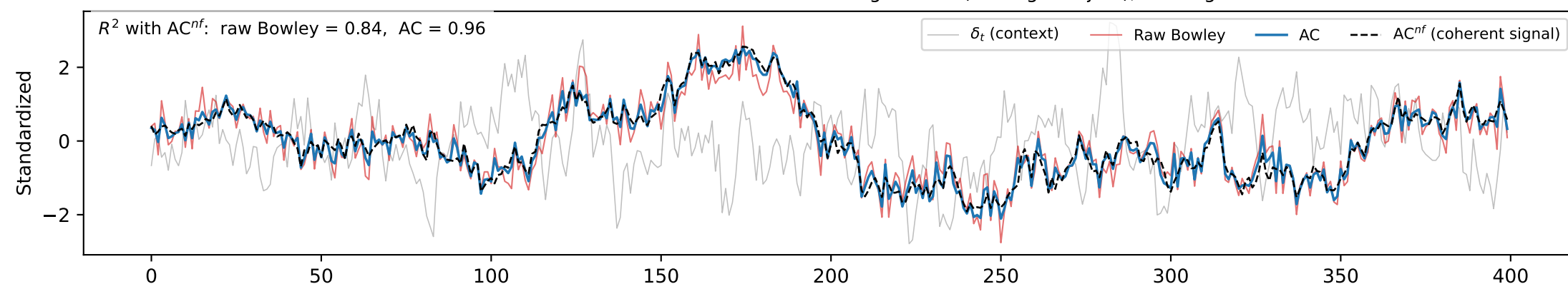
Panel C: Third moment — AC tracks the noise-free coherent signal AC^{nf} (its target object), filtering incoherent noise
