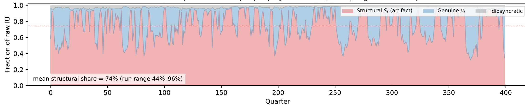
Panel D: Exact decomposition of raw IU_t = S_t + u_t + I_t — structural (artifact) vs genuine vs idiosyncratic
