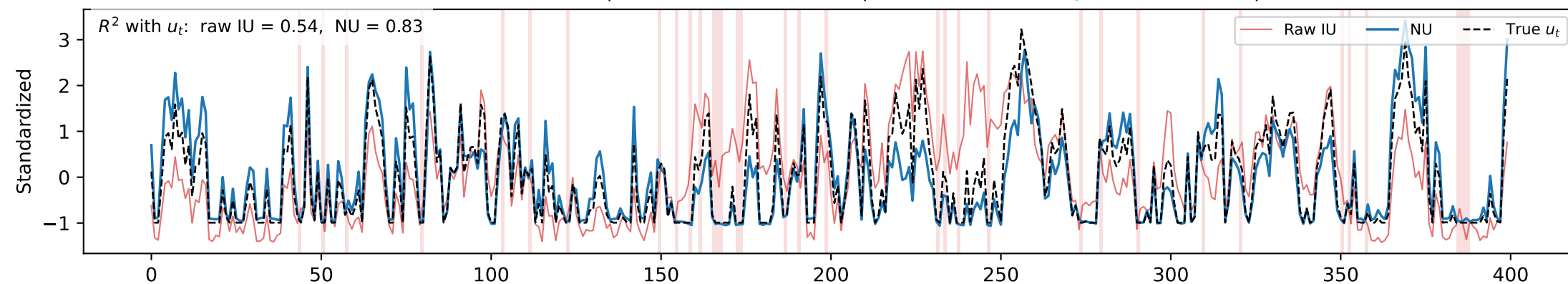
Panel B: Second moment — in shaded episodes the structural component moves while u_t is stable; raw IU spikes, NU does not
