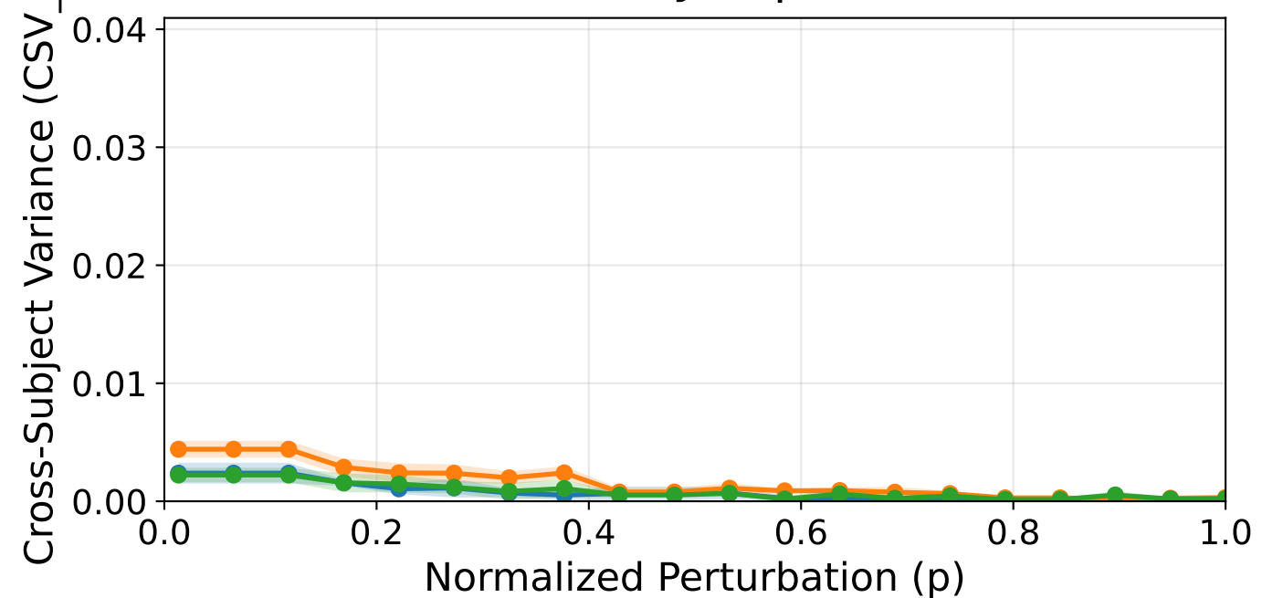
Cross-Subject | Tuned
