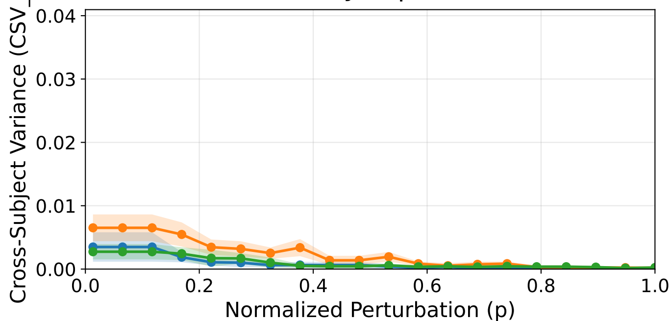
Cross-Subject | Baseline
