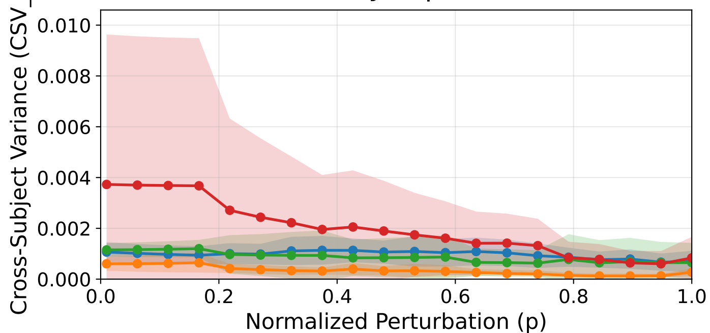
Cross-Subject | Baseline
