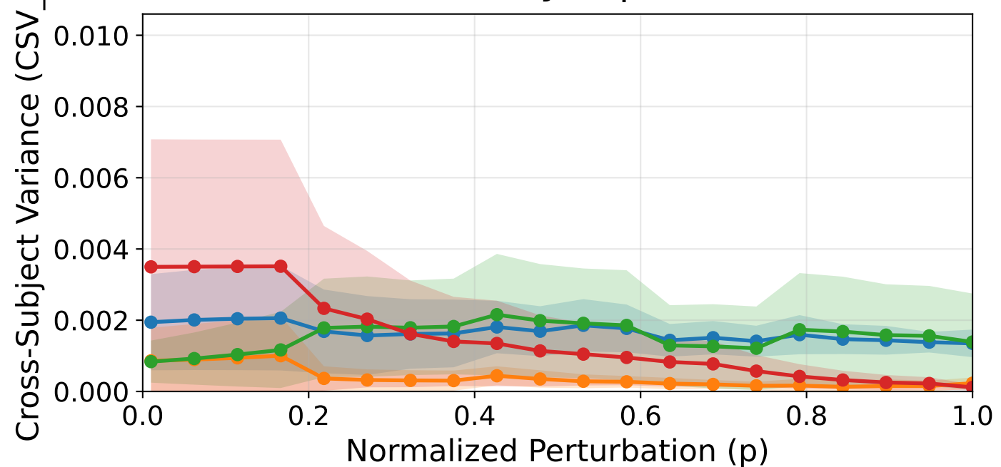
Cross-Subject | Tuned
