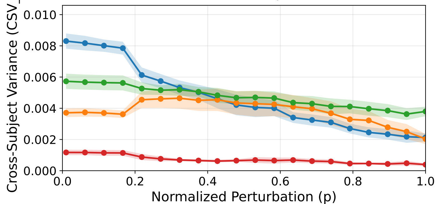
Cross-Subject | Tuned
