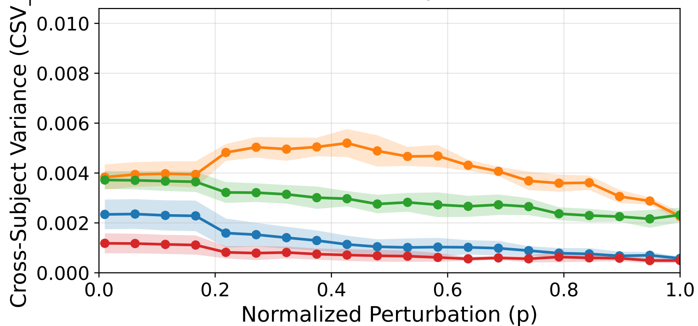
Cross-Subject | Baseline
