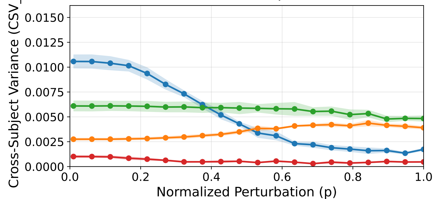
Cross-Subject | Tuned
