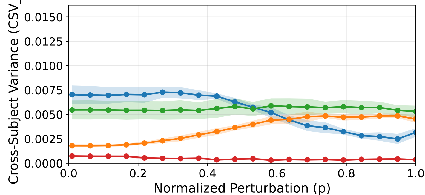
Within-Session | Tuned
