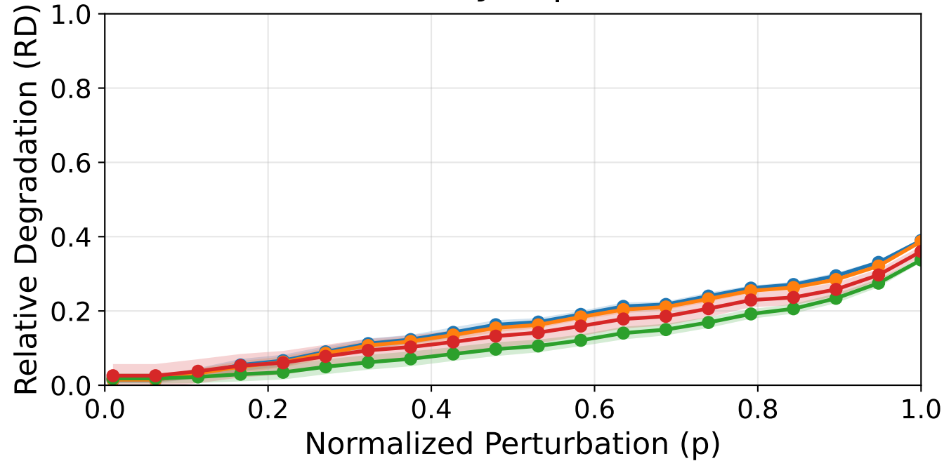
Cross-Subject | Baseline
