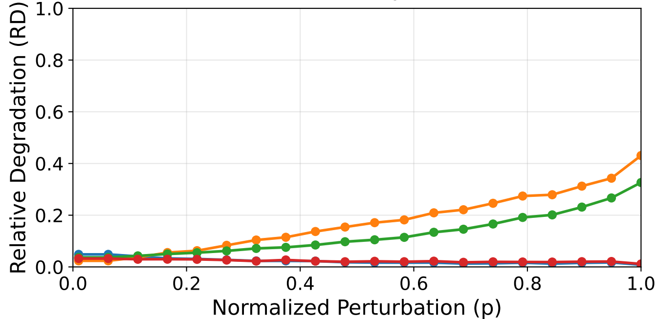
Cross-Subject | Baseline
