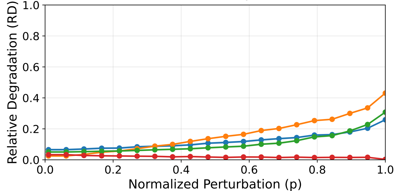
Cross-Subject | Tuned
