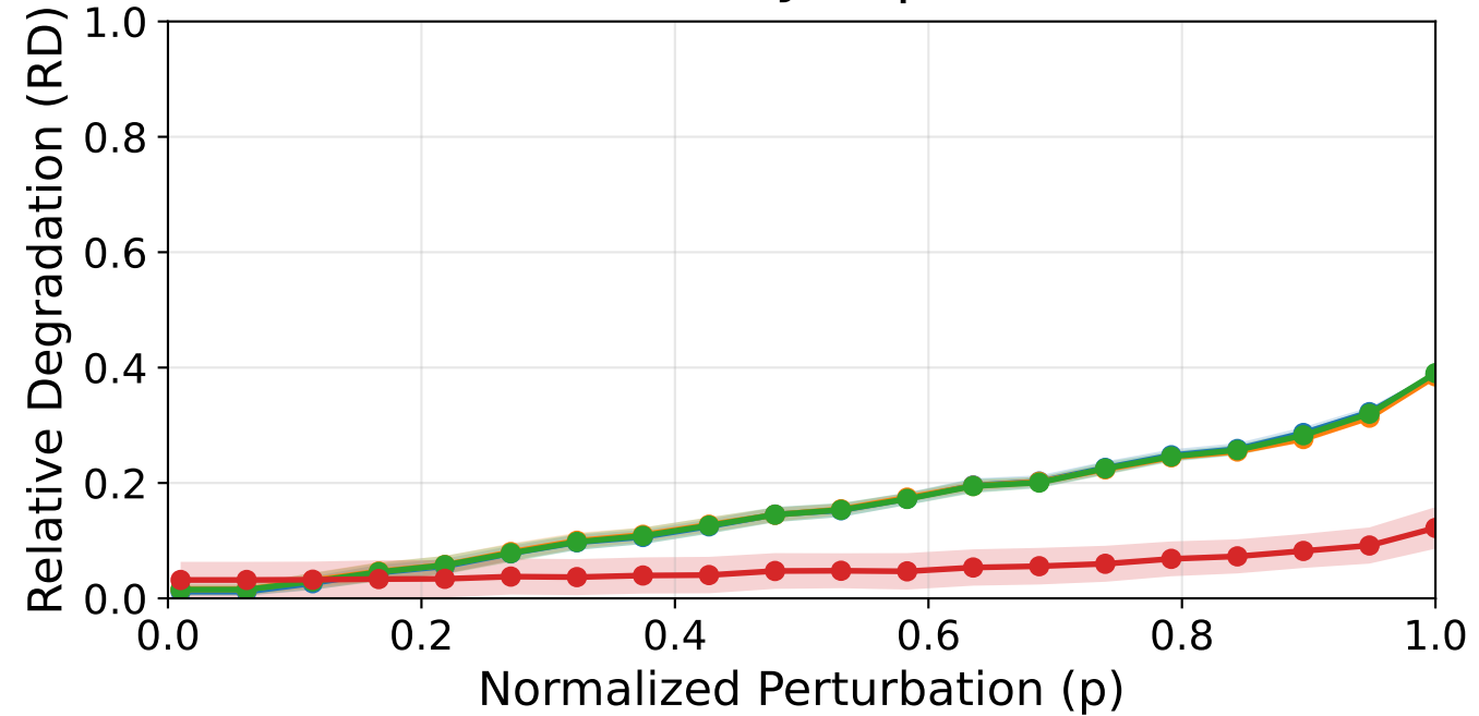
Cross-Subject | Tuned
