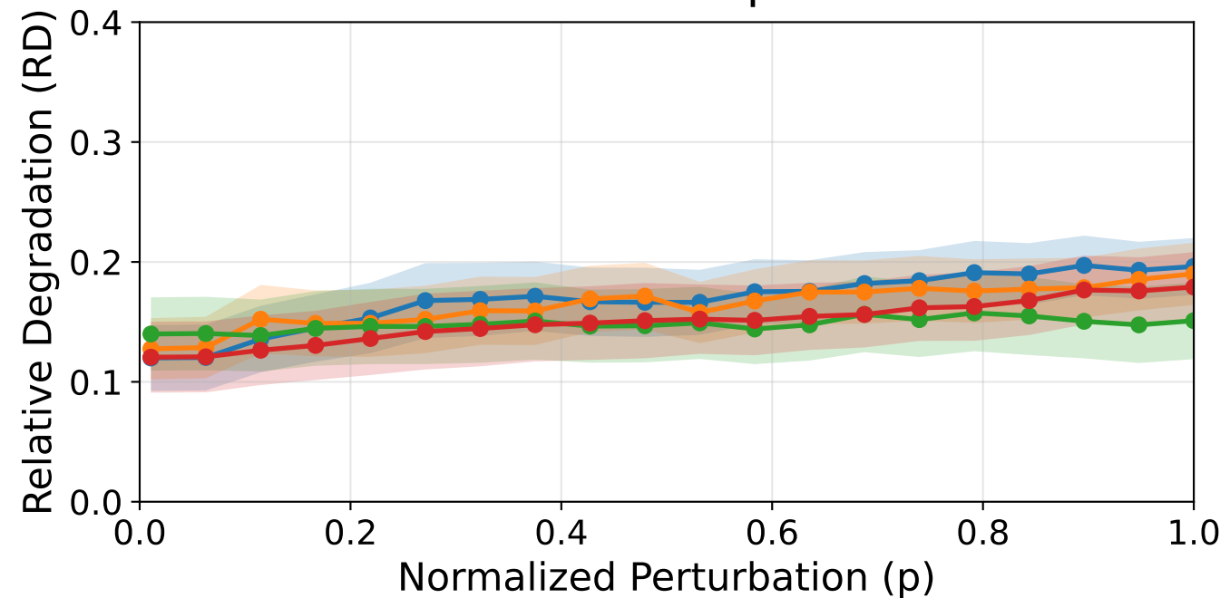
Within-Session | Tuned
