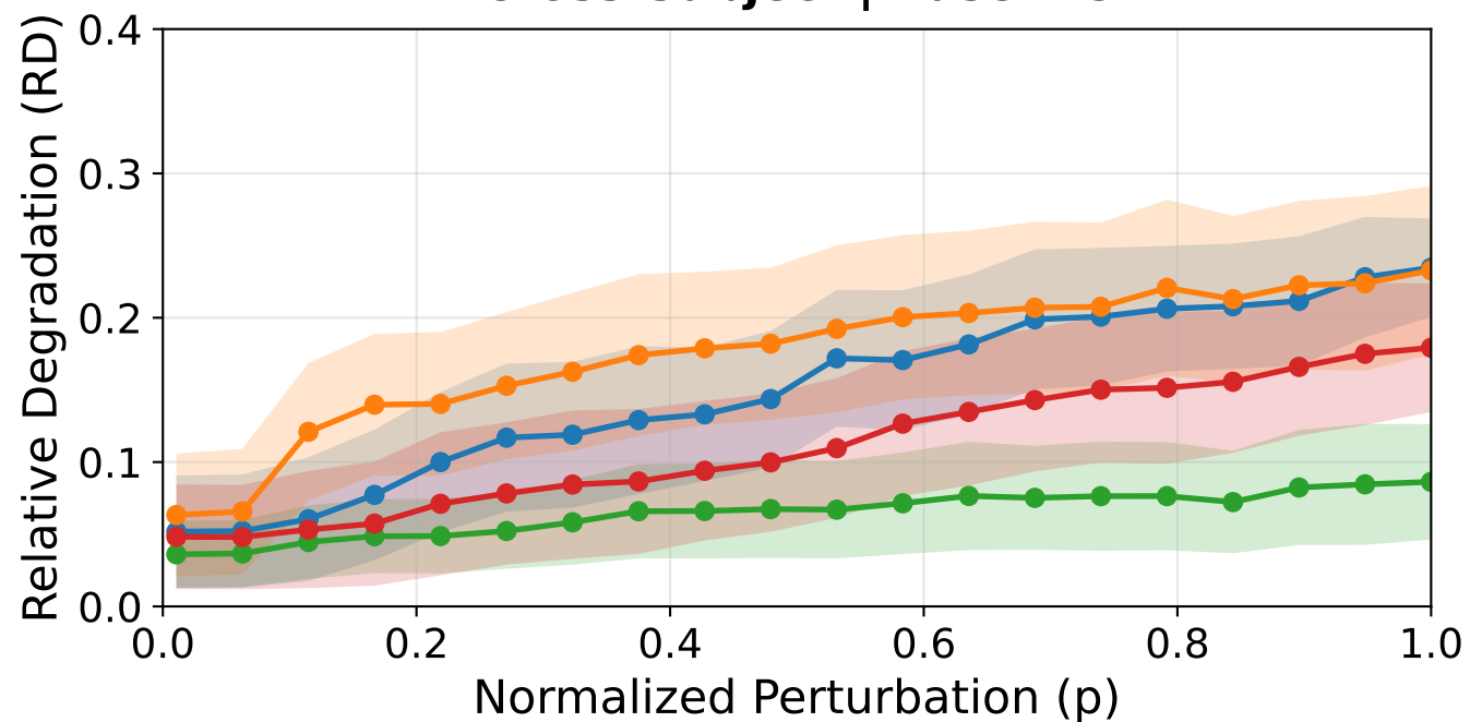
Cross-Subject | Baseline
