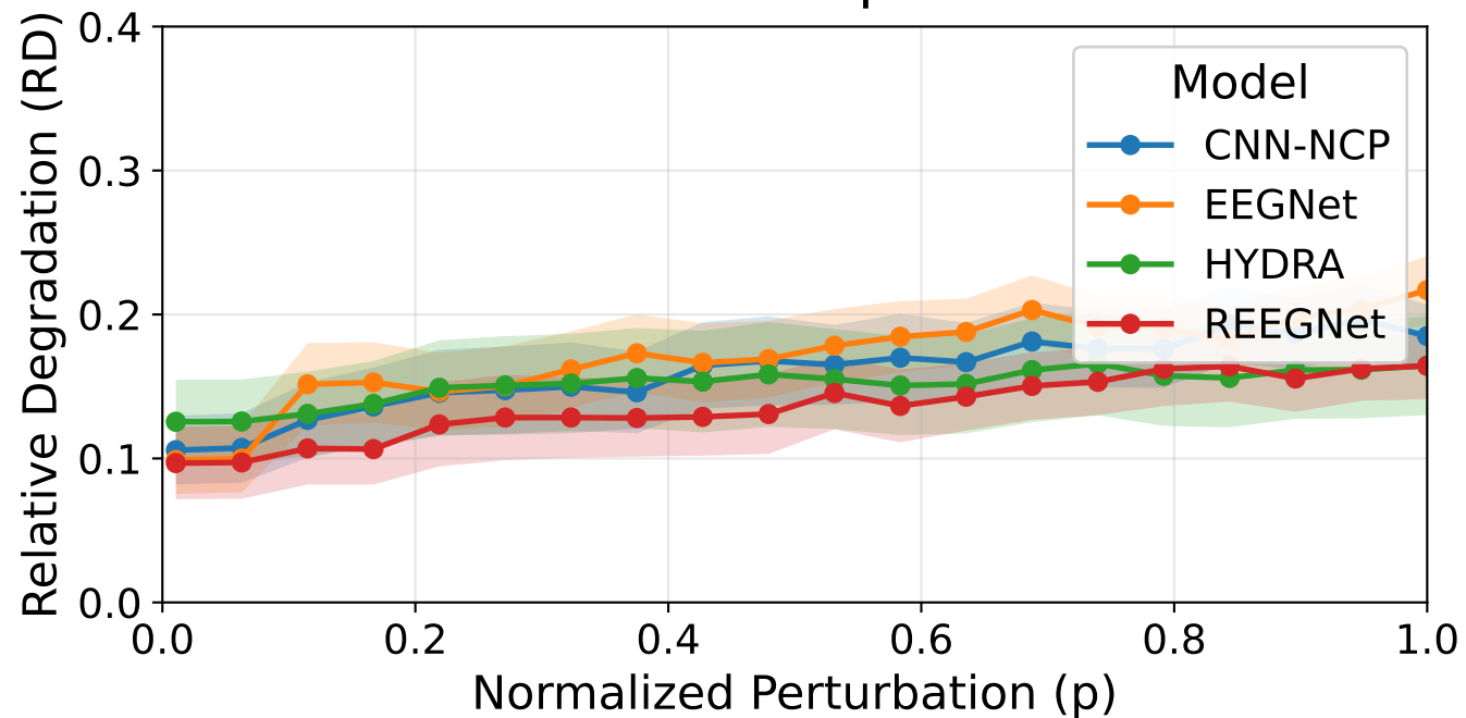
Within-Session | Baseline
