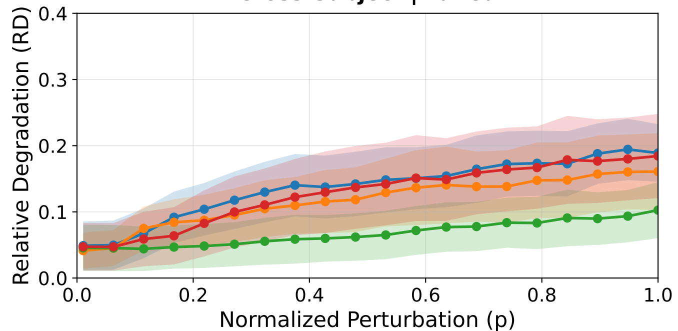
Cross-Subject | Tuned
