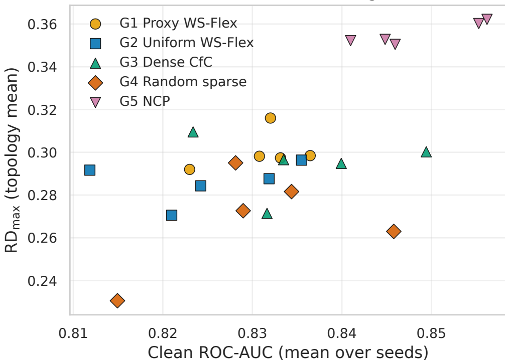
Clean ROC-AUC vs. Relative Degradation
