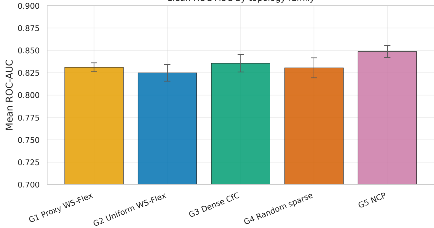
Clean ROC-AUC by topology family
