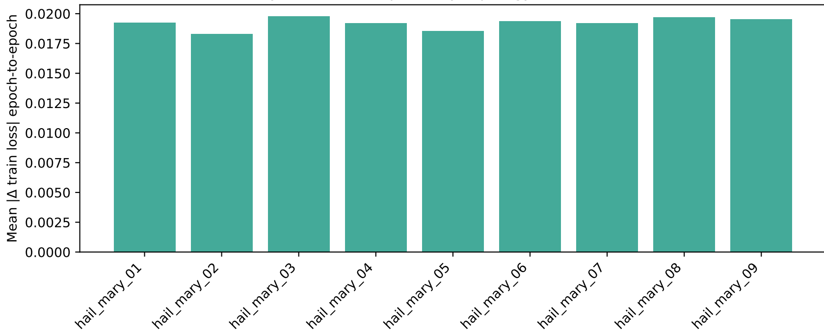
Hail Mary: train loss step size by topology (mean across seeds)
