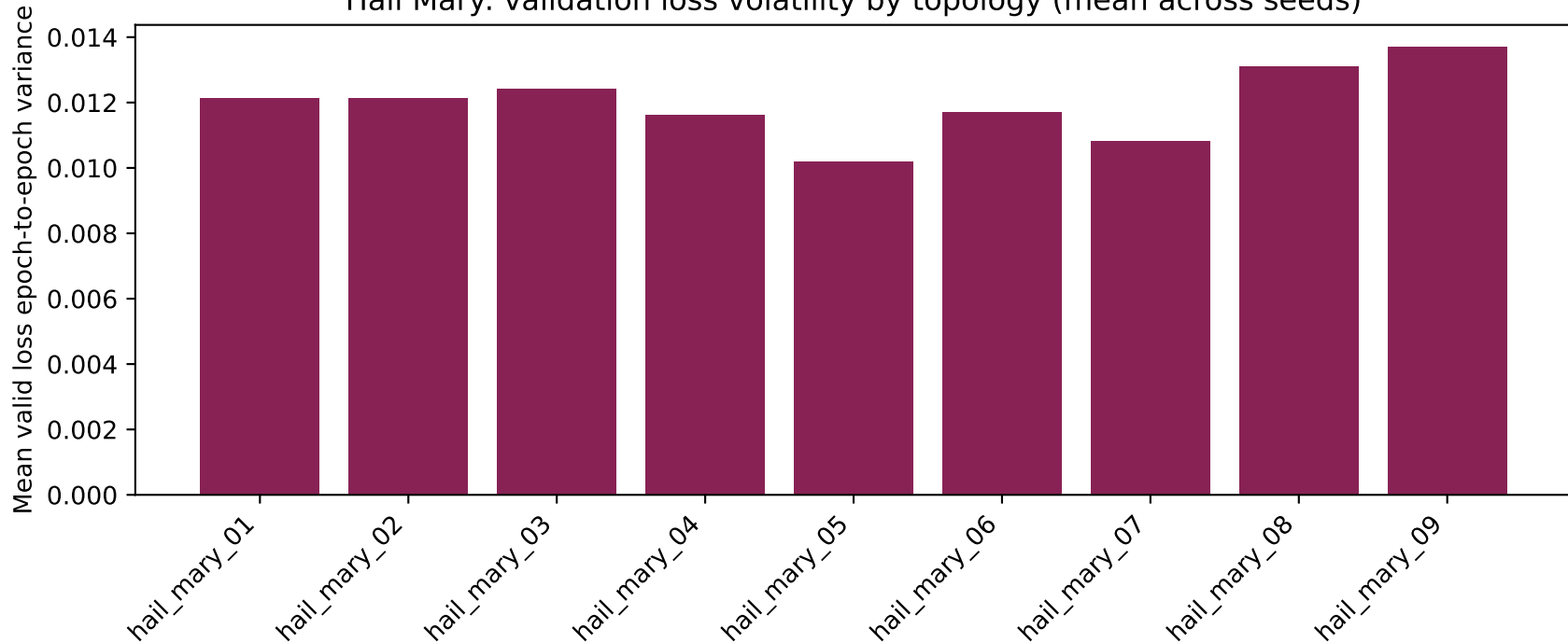
Hail Mary: validation loss volatility by topology (mean across seeds)
