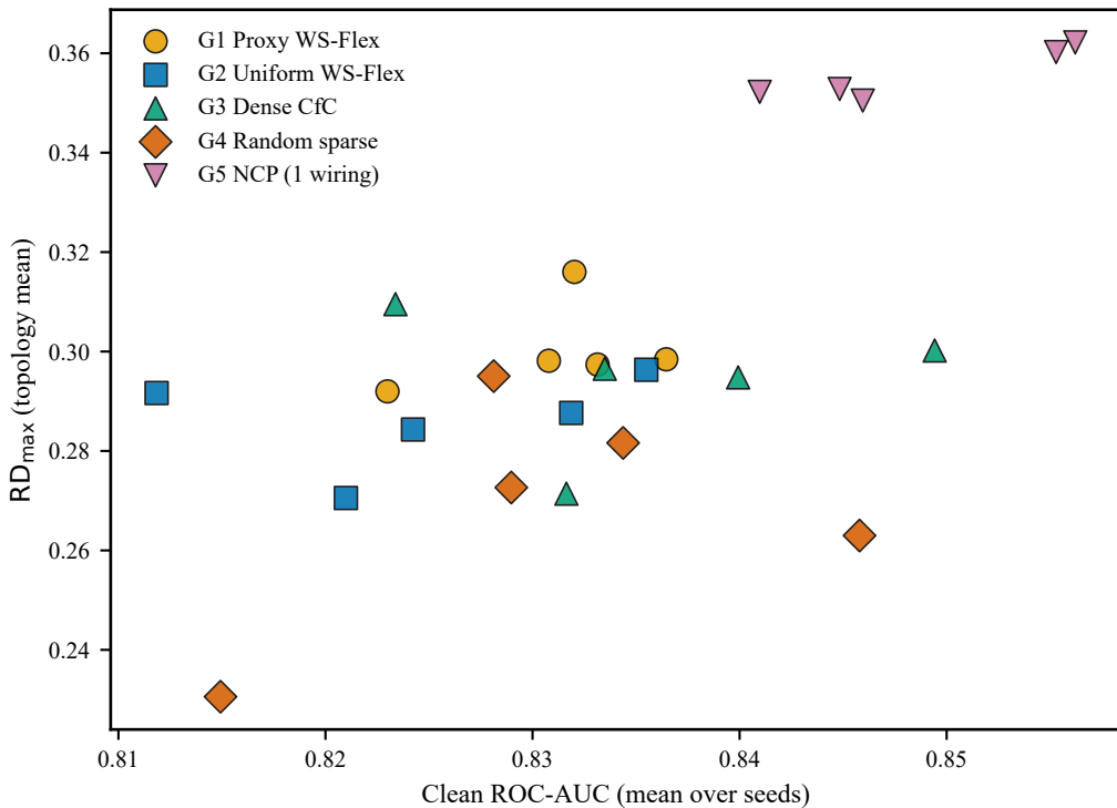
Clean performance vs robustness
