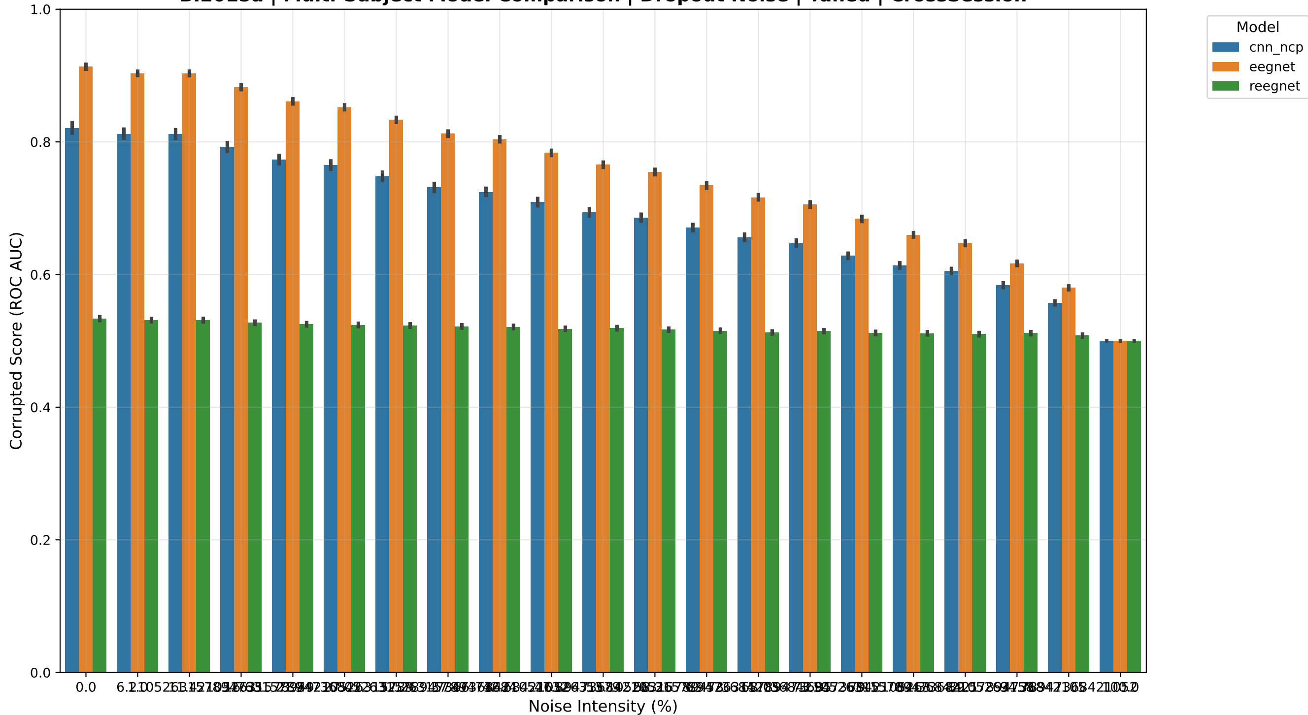
BI2015a | Multi-Subject Model Comparison | Dropout Noise | Tuned | CrossSession
