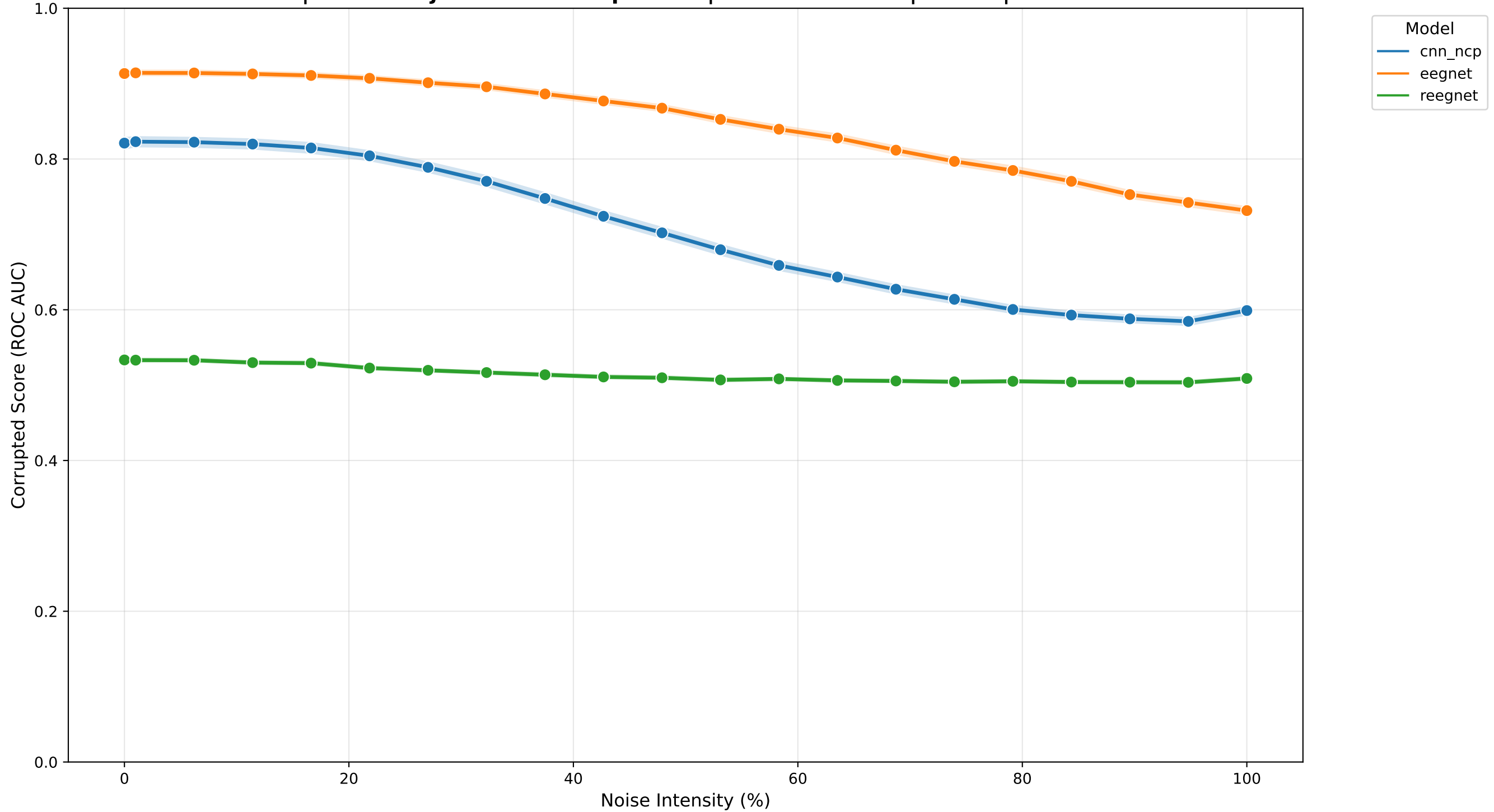
BI2015a | Multi-Subject Model Comparison | Gaussian Noise | Tuned | CrossSession
