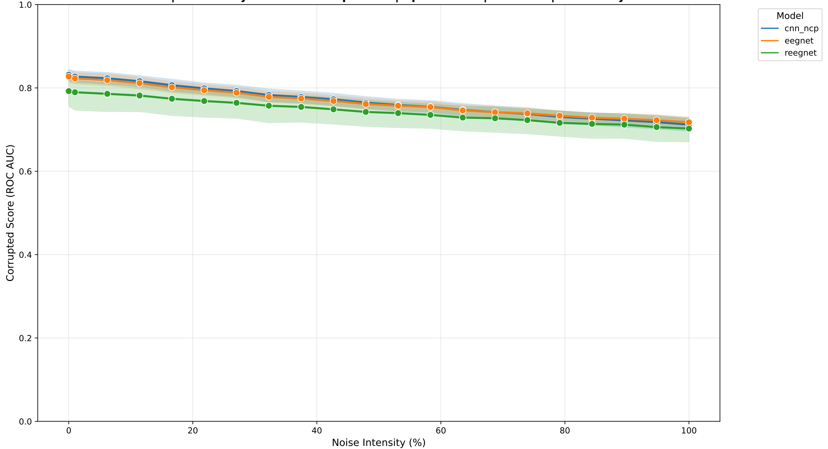
BI2015a | Multi-Subject Model Comparison | Spike Noise | Baseline | CrossSubject
