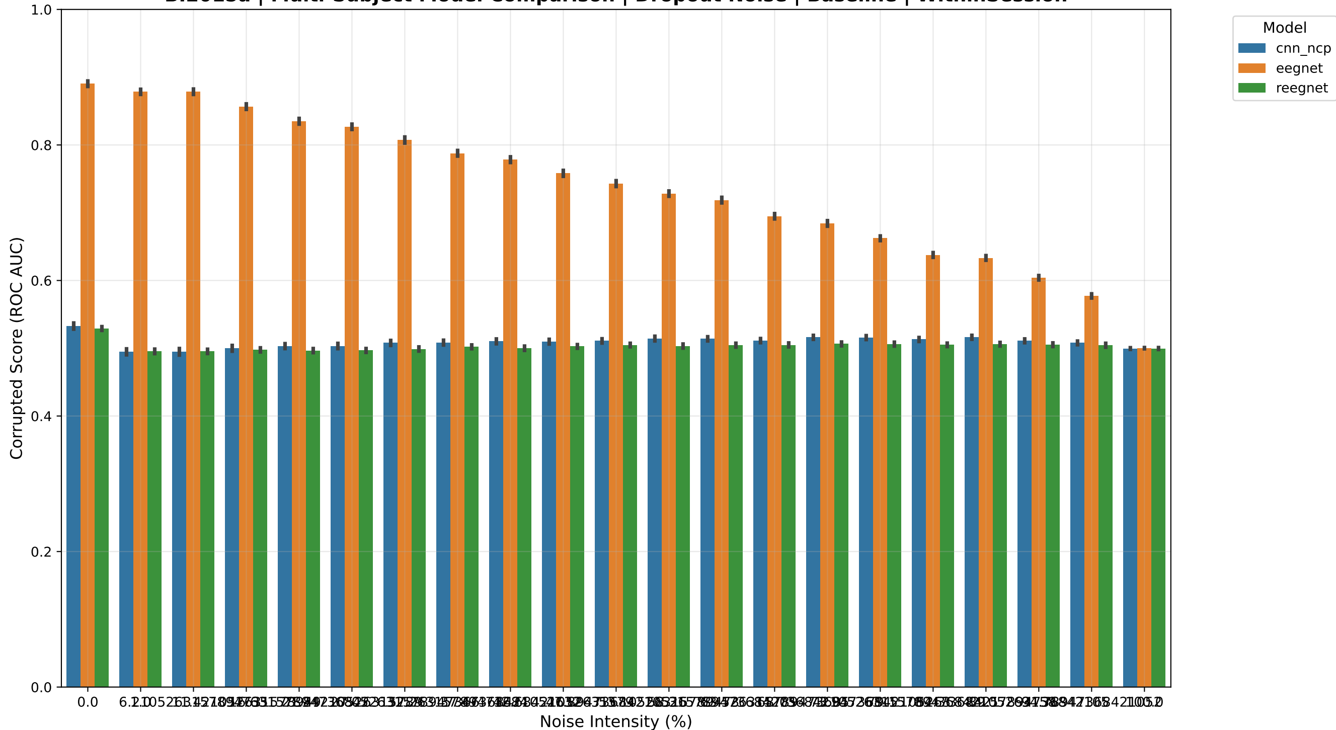
BI2015a | Multi-Subject Model Comparison | Dropout Noise | Baseline | WithinSession
