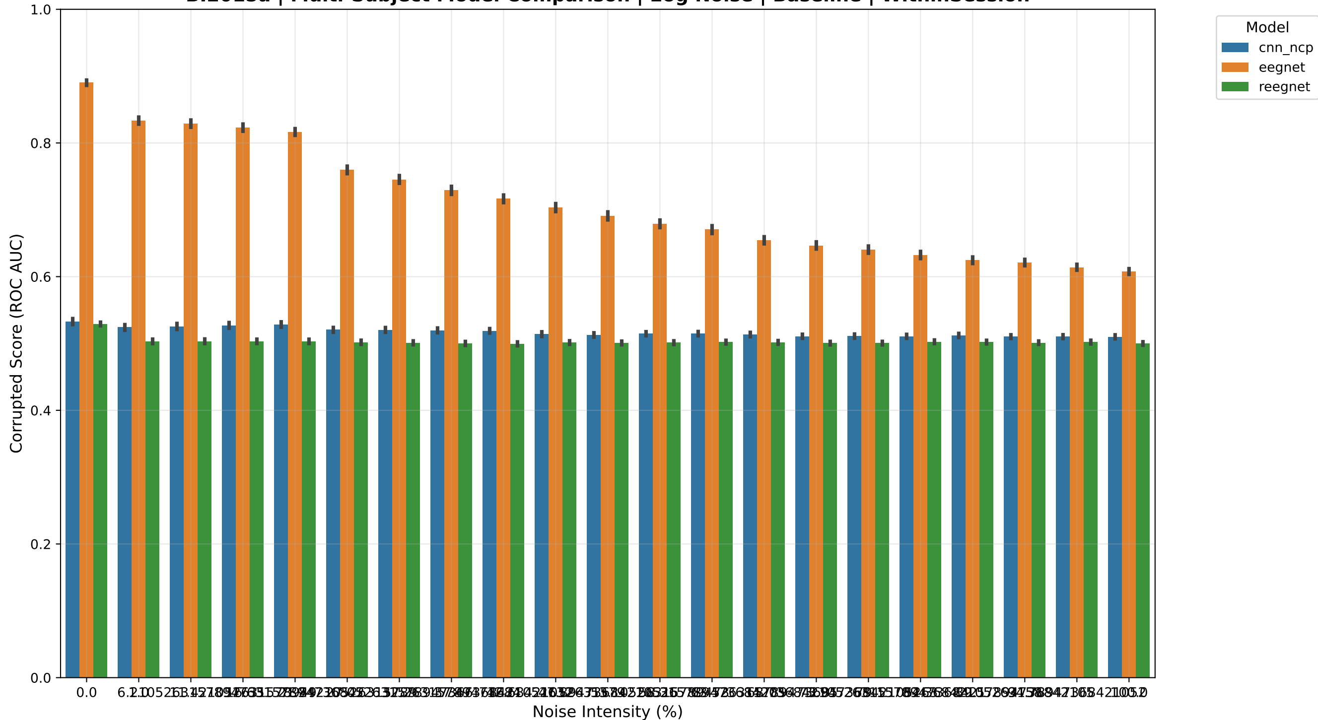
BI2015a | Multi-Subject Model Comparison | Eog Noise | Baseline | WithinSession
