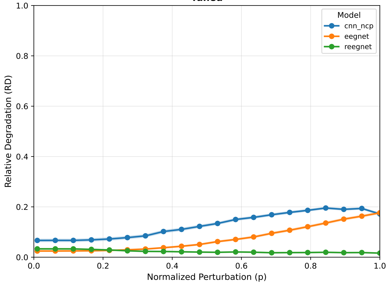
Tuned
