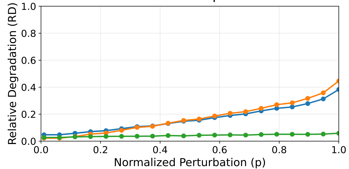
Within-Session | Tuned
