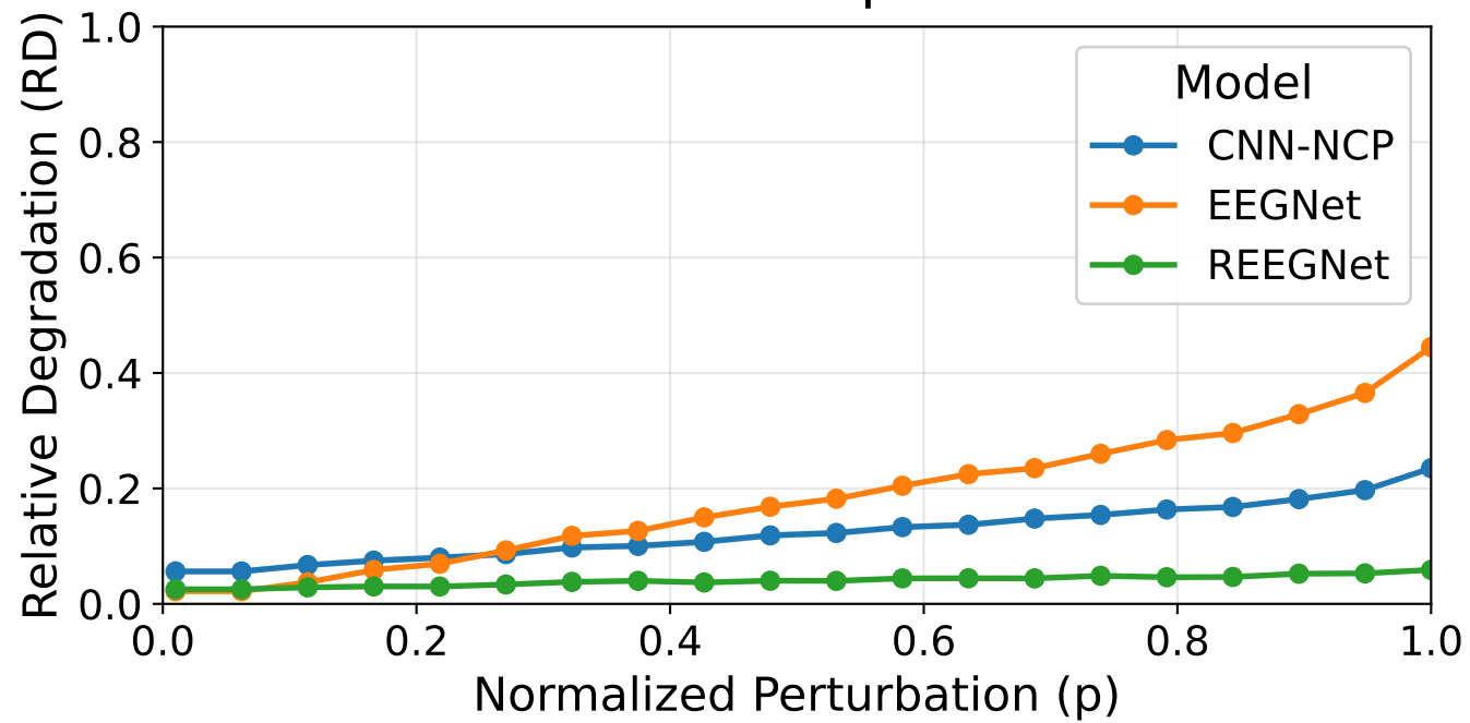
Within-Session | Baseline
