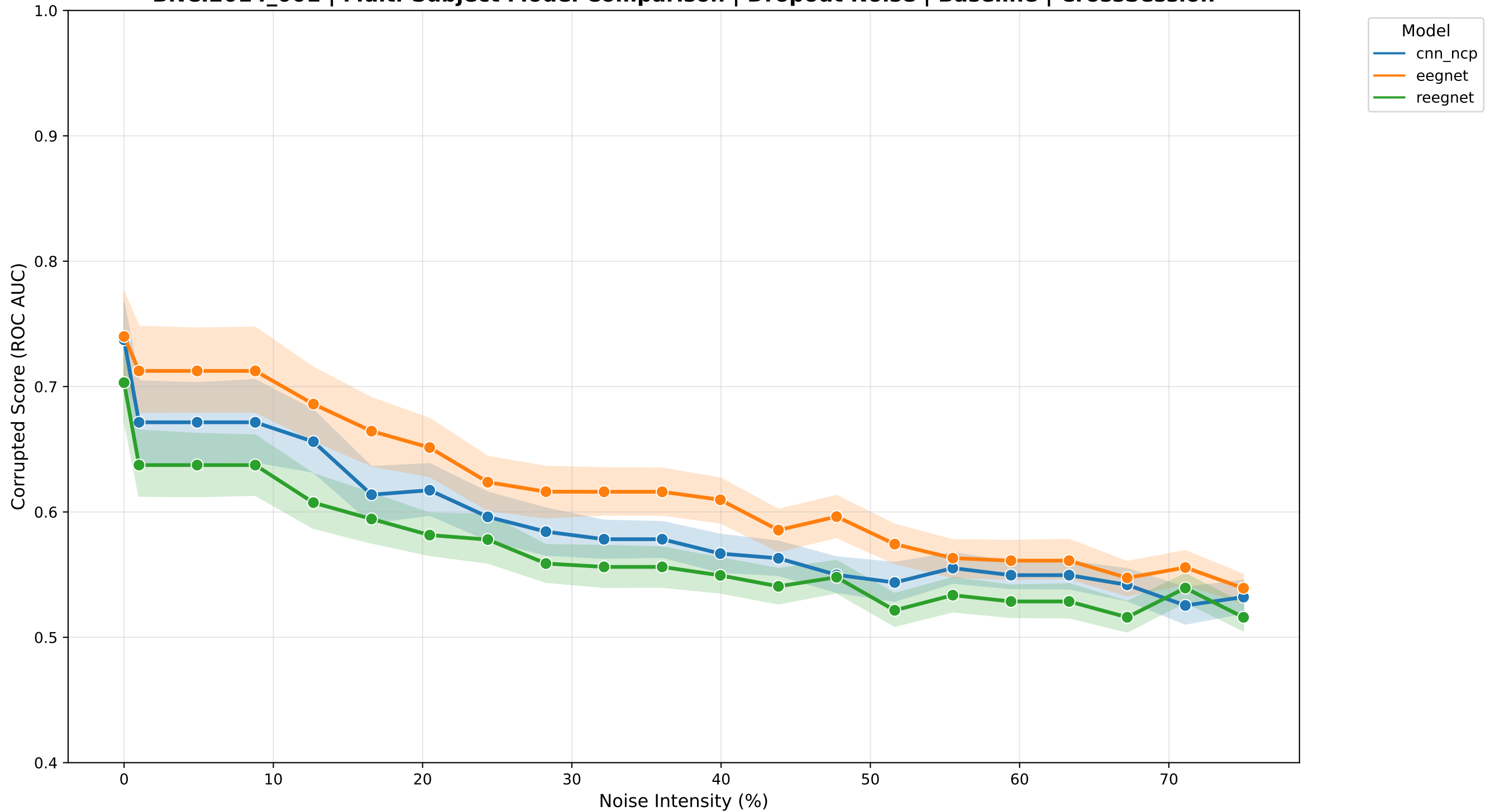
BNCI2014_001 | Multi-Subject Model Comparison | Dropout Noise | Baseline | CrossSession
