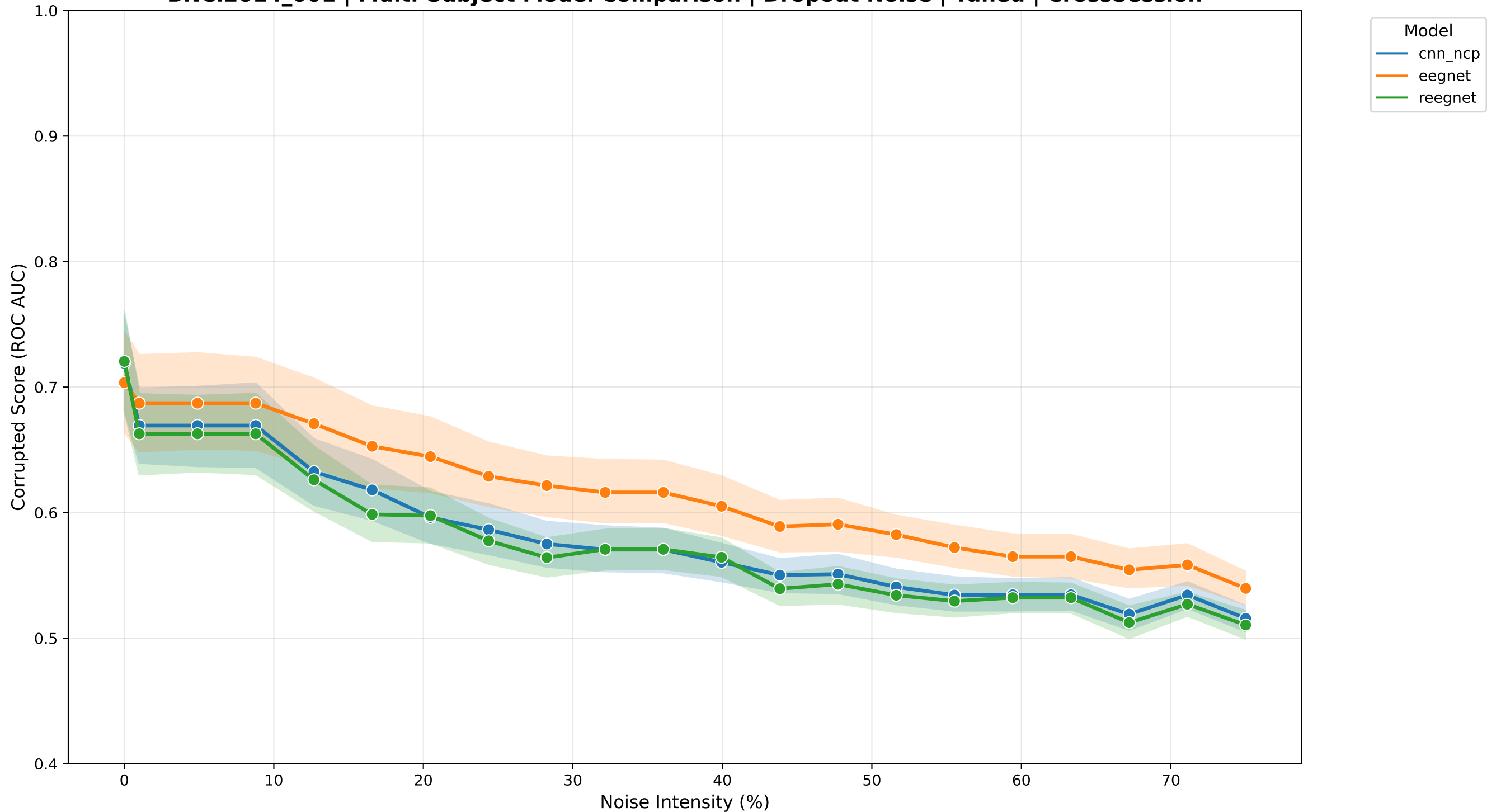
BNCI2014_001 | Multi-Subject Model Comparison | Dropout Noise | Tuned | CrossSession
