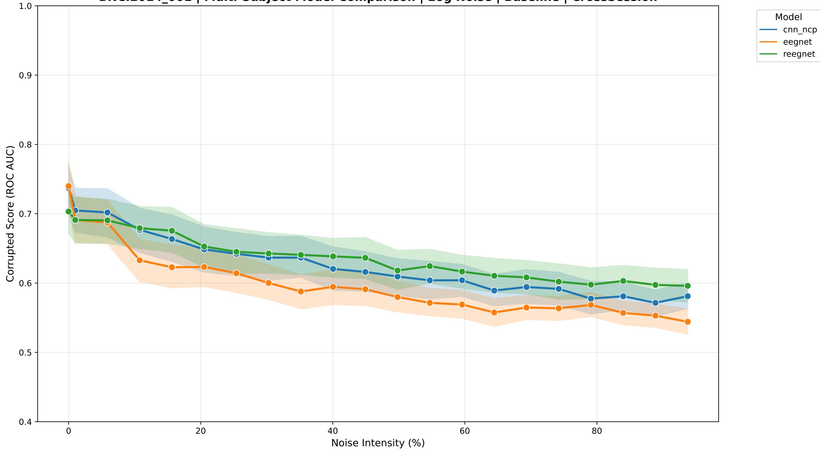
BNCI2014_001 | Multi-Subject Model Comparison | Eog Noise | Baseline | CrossSession
