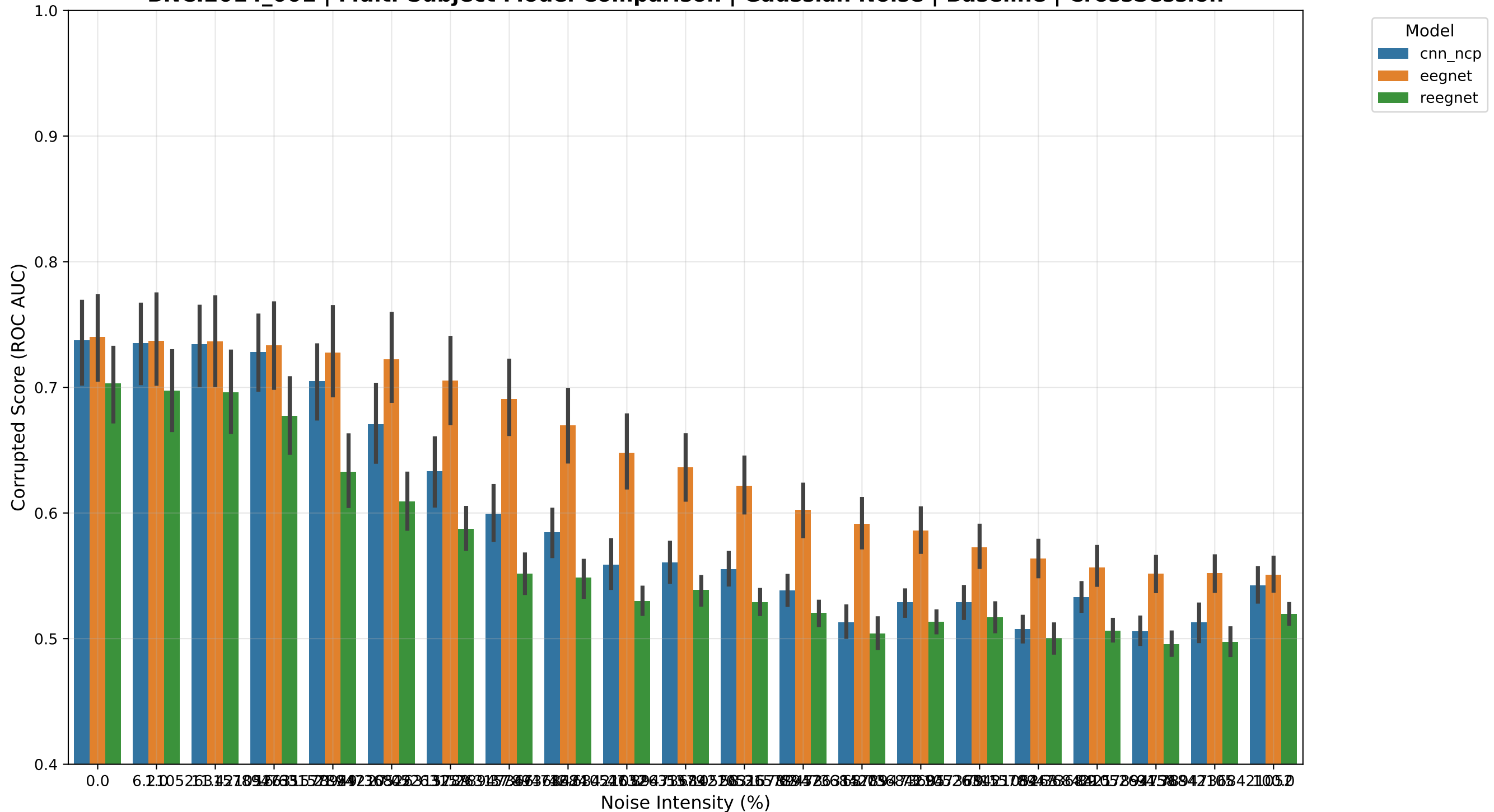
BNCI2014_001 | Multi-Subject Model Comparison | Gaussian Noise | Baseline | CrossSession
