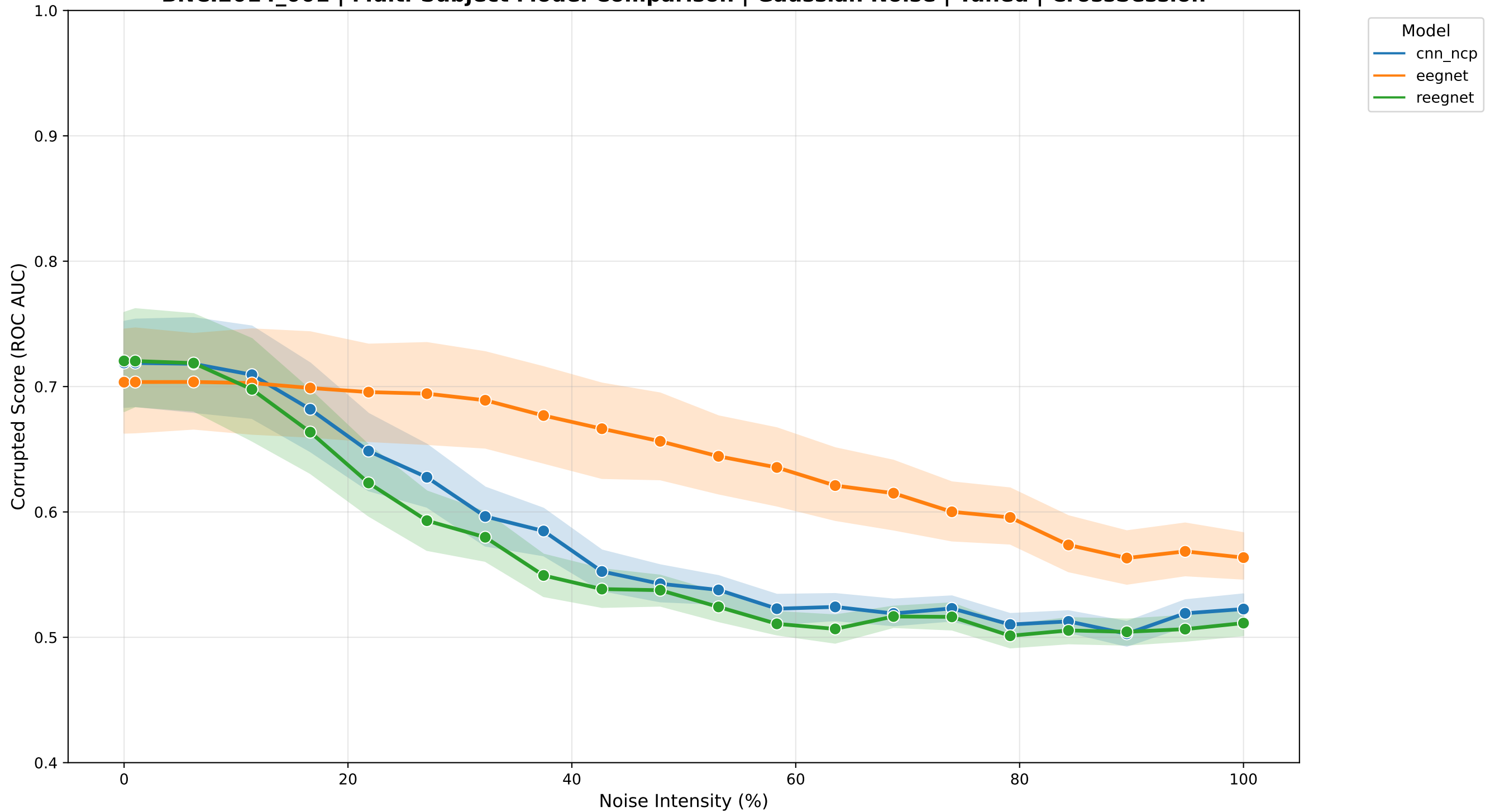
BNCI2014_001 | Multi-Subject Model Comparison | Gaussian Noise | Tuned | CrossSession
