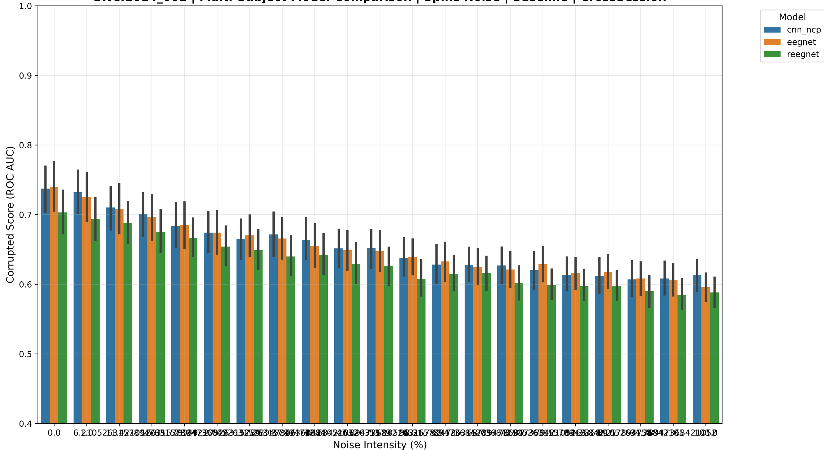
BNCI2014_001 | Multi-Subject Model Comparison | Spike Noise | Baseline | CrossSession
