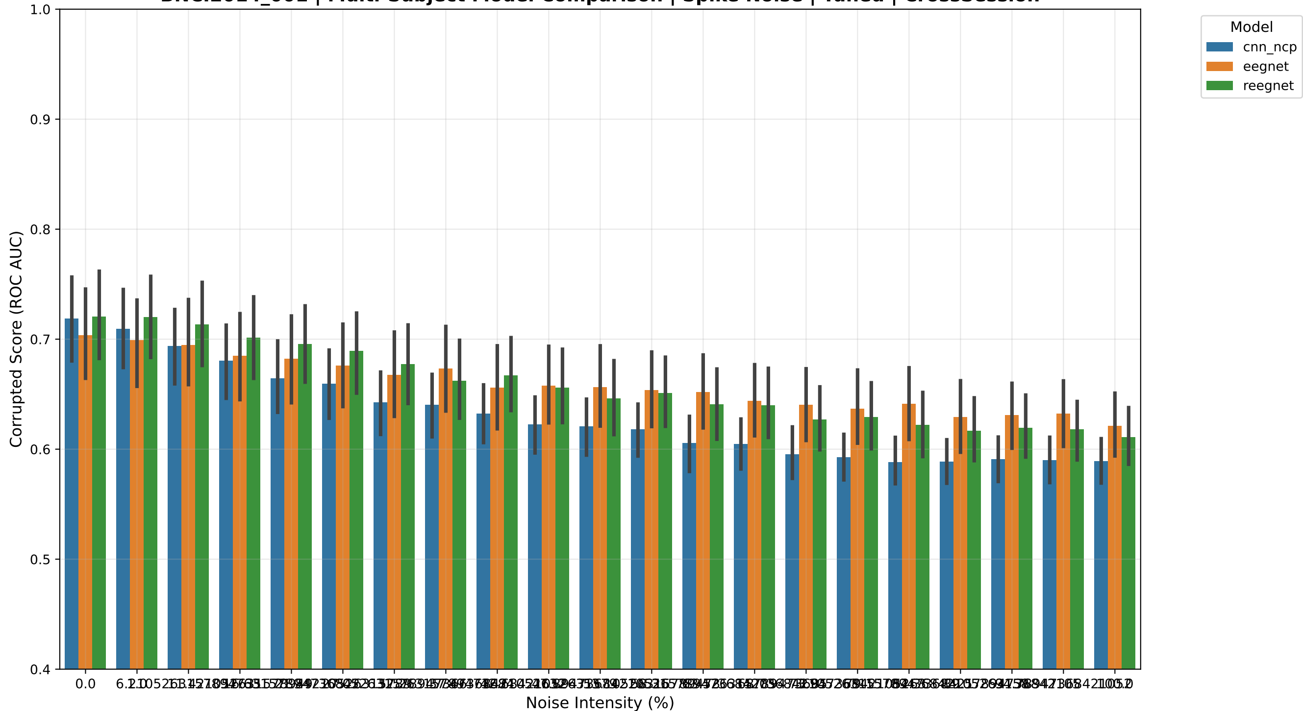
BNCI2014_001 | Multi-Subject Model Comparison | Spike Noise | Tuned | CrossSession
